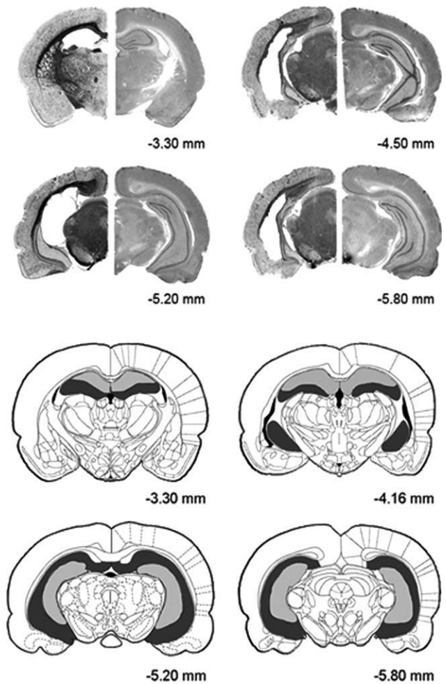
FIGURE 8. (A) Photomicrographs of coronal sections of a representative hippocampal lesion (left) in relation to a normal brain (right) and (B) schematic drawings of minimal (gray) and maximal (black) extents of lesions. The numbers represent the distance in millimeters posterior to bregma.
